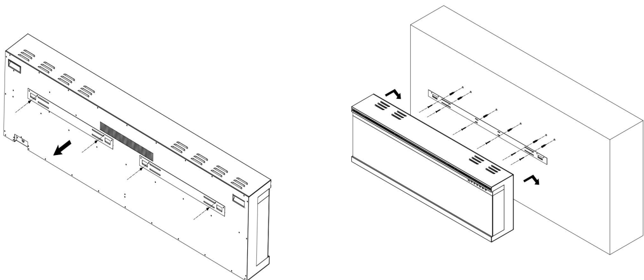
UNIQUE 180 PRO Wall Bracket Illustrated
